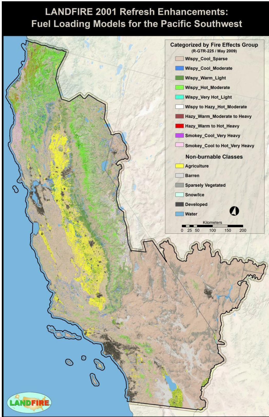
Figure 14 – LF 2001 Fuel Loading Models for the PSW GeoArea. FLM categories are from Rocky Mountain Research Station General Technical Report 225.
