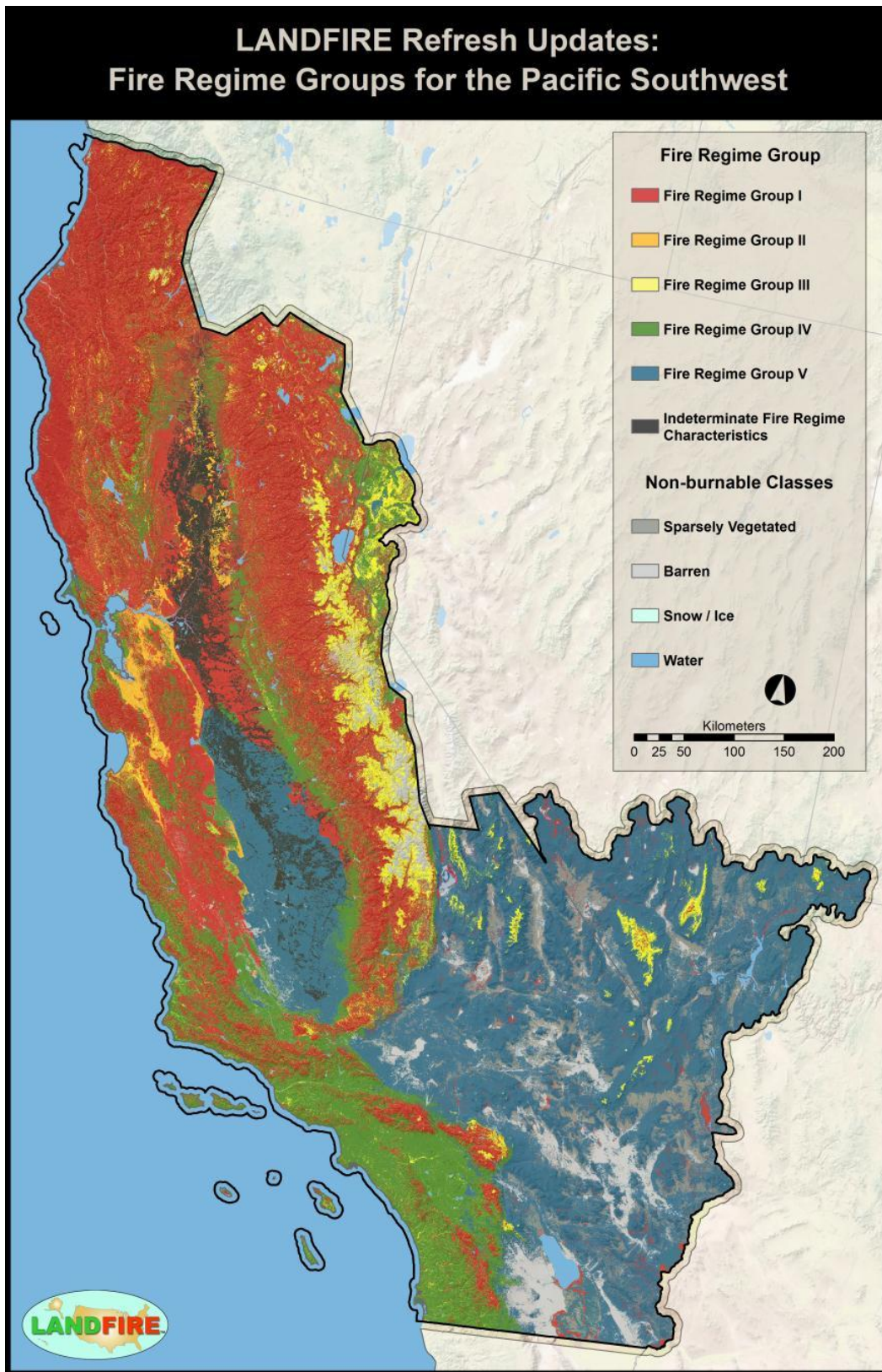
Figure 4 – Map of the PSW landscape depicting LF Fire Regime Groups in the absence of modern human intervention with possible aboriginal fire use.
