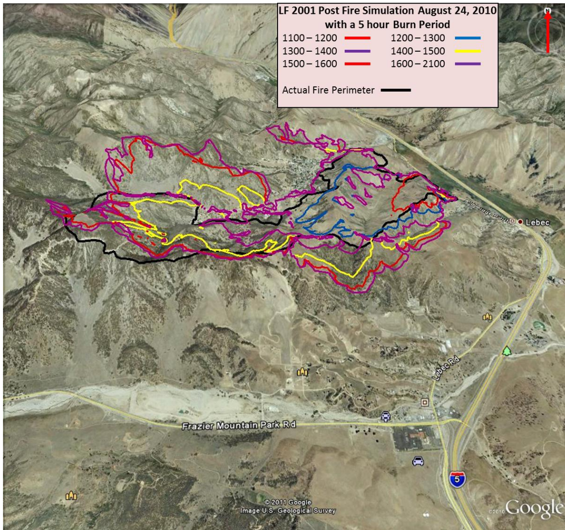
Figure 28 – LF 2001 fuels in the Post Fire simulation. The red, blue, yellow, and purple perimeter lines show the extent of the fire at different time periods during the fire. The black lines show the final perimeter of the Post Fire. The fire spread perimeter extends nearly 3 miles southwest to northeast.
