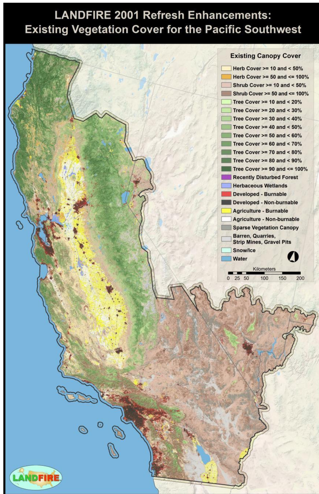
Figure 7 – Map of Existing Vegetation Cover layer that was enhanced as part of the LF 2001 update by incorporating user feedback and additional data.
