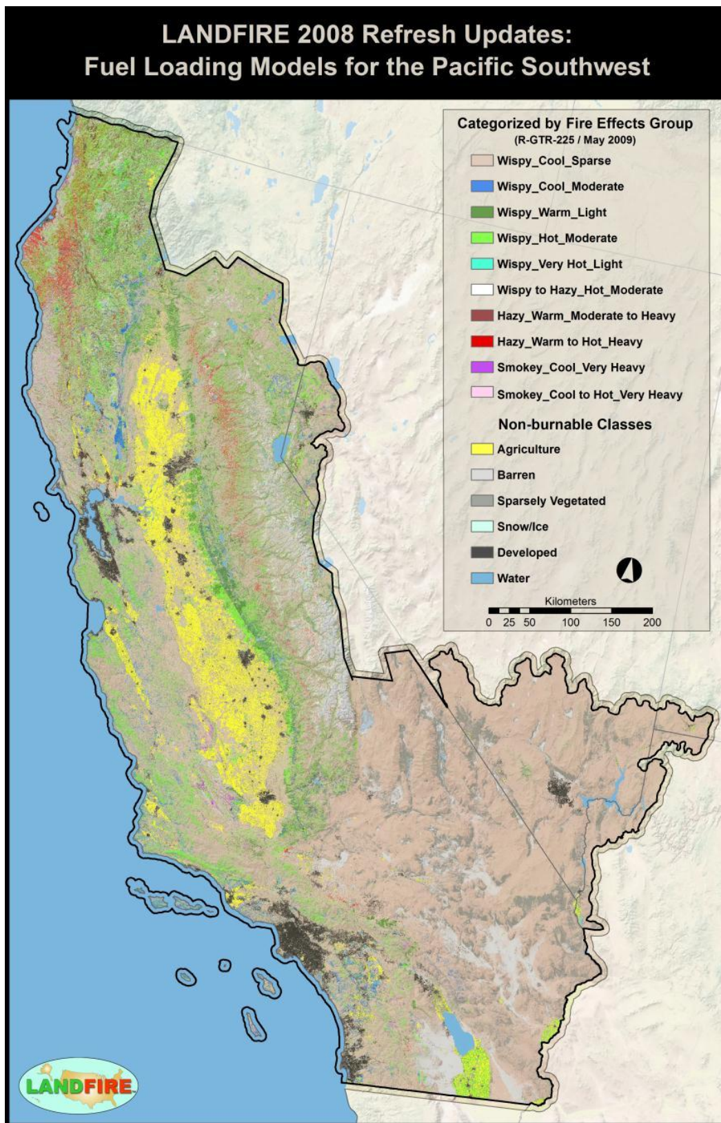
Figure 15 – LF 2008 Fuel Loading Models for the PSW GeoArea. Categories are from the Rocky Mountain Research Station General Technical Report 225.
