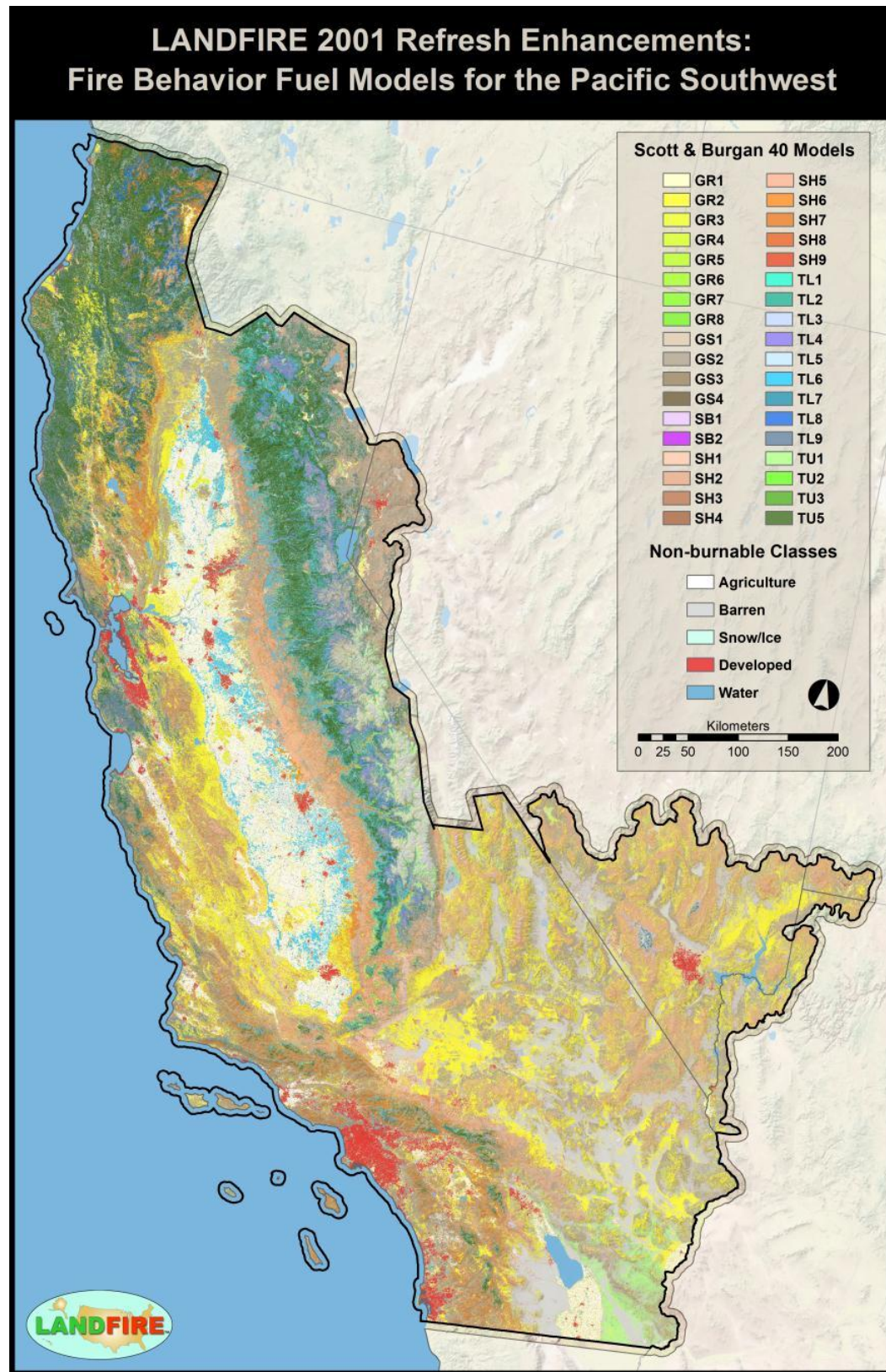
Figure 12 – LF 2001 FBFM40 for the PSW GeoArea.
