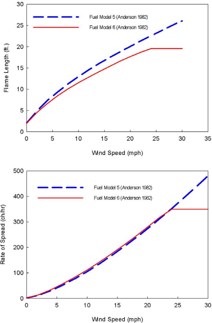
Figure 4. Comparison of rate of spread and flame length of fire behavior fuel models 5 and 6 (Anderson 1982). The moisture scenario assumes fine dead fuel moistures of 3, 4, and 5 percent for 1-, 10-, and 100-hour time-lag fuel, respectively. Herbaceous moisture is assumed to be 30 percent, whereas the moisture content of live woody fuel is assumed to be 60 percent. Under these conditions, either fuel model could be used to describe the observed or expected fire behavior.
