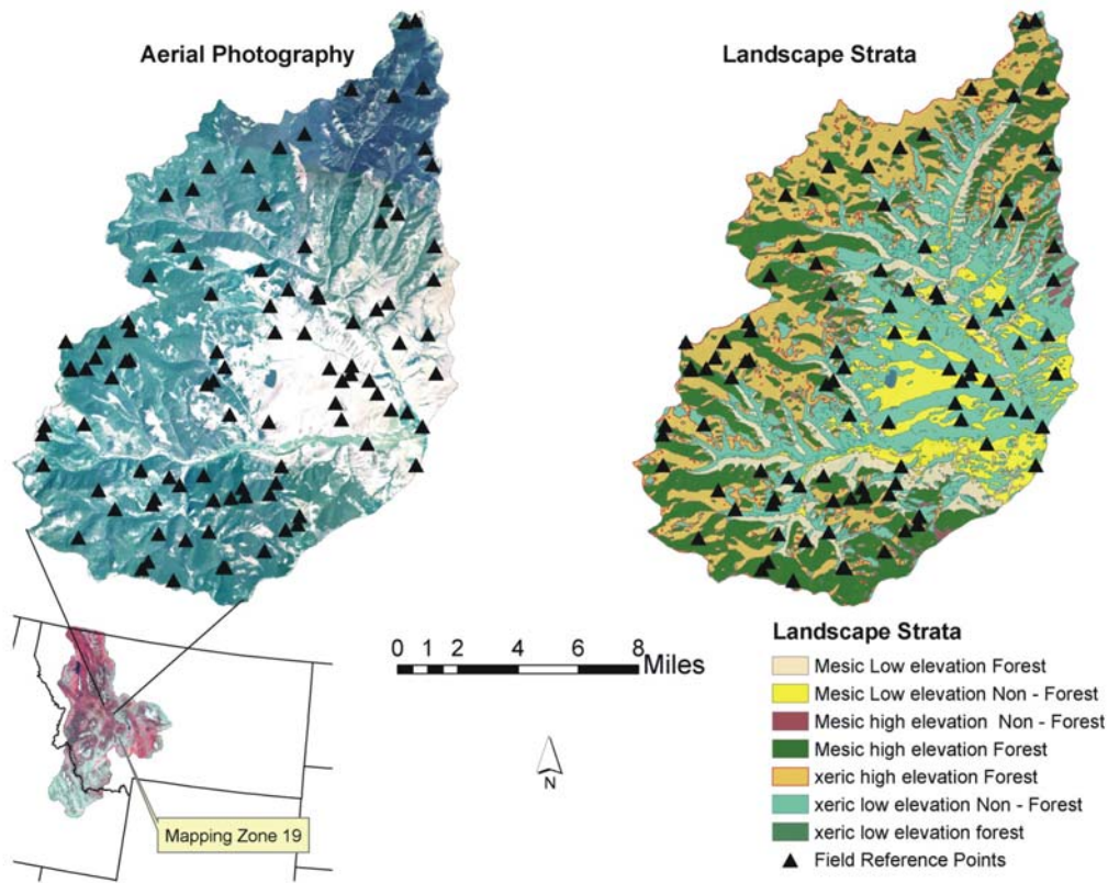
Figure 3. Location and land strata of a 5 th code hydrologic unit code (HUC) in LANDFIRE Mapping Zone 19 used to exemplify a suggested method of evaluating LANDFIRE fuel data. Black triangles represent the central location of 100 field reference points located using a stratified random sampling approach. Four other points were taken 100 meters from the central point. Care was taken to locate the points far from strata boundaries. The number of points in each stratum is commensurate with the acreage each strata covers (see table 2 below).
